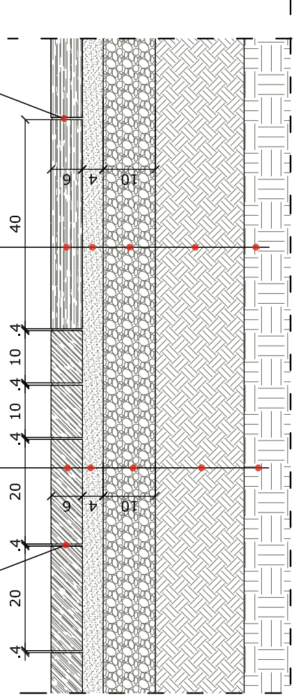
DETALIU D7 : ALEE PIETONALA DALE BETON - DALE BETON ZONA SKATE
